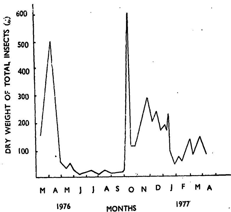
Fig. 1 (a). Dry weight of total light trap catch at Maha Illuppallama (includes all species)
