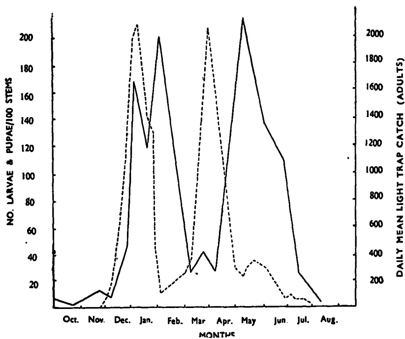
Fig. 2. Population of the stem-borer, Chilo partellus at Maha Iluppallama (1976-79)
