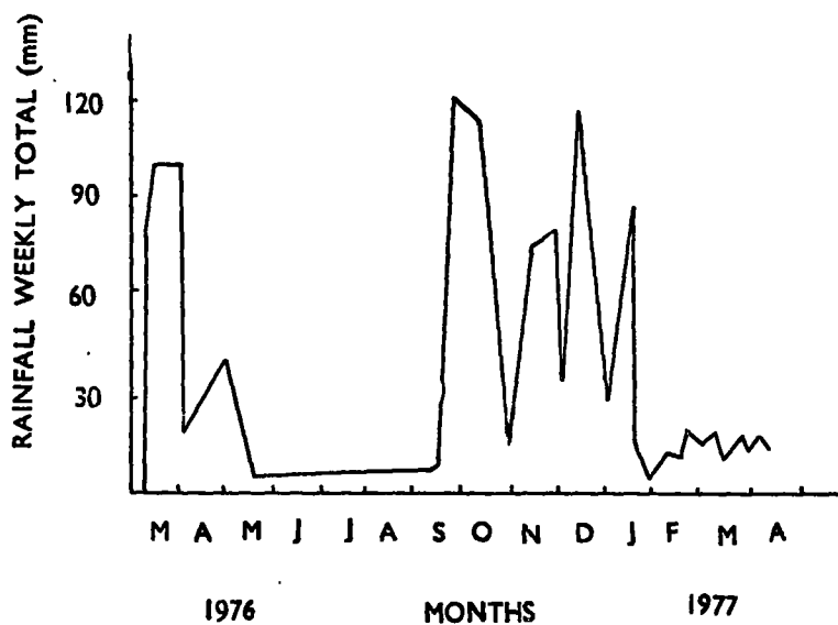
Fig. 1 (b). Weekly rainfall distribution at Maha Illuppallama during 1976-77
