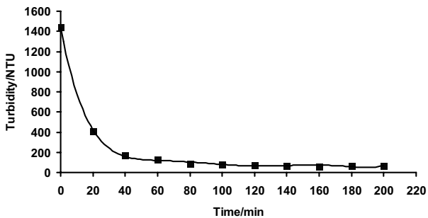
Figure 5: Variation of turbidity of the supernatant solution of brick particle - Cr(VI) suspension with settling time ( d < 1 mm, 10 g brick clay fired at 200 °C, 100.0 cm 3 solution, 10 min stirring time).
