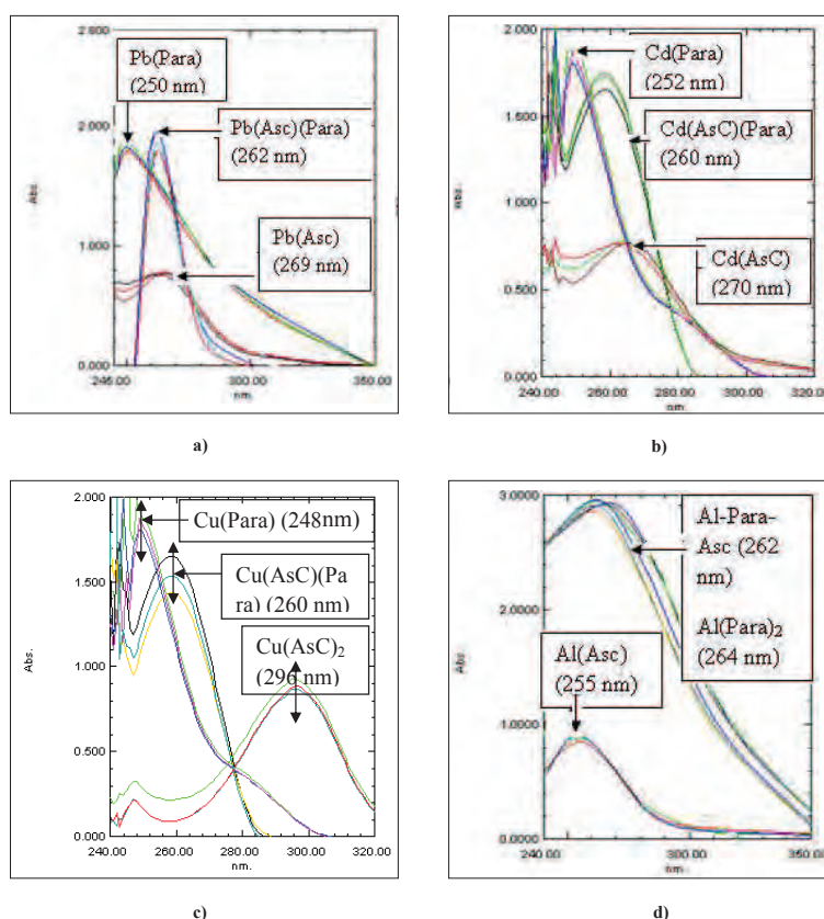
Figure 3: Comparison of UV absorption spectra of binary and mixed ligand systems: (a) Pb(Para), Pb(Asc)(Para), Pb(Asc) (b) Cd(Para), Cd(Asc)(Para), Cd(Asc); (c) Cu(Para), Cu(Asc)(Para), Cu(Asc) 2 ; (d) Al(Para) 2 , Al-Asc-Para, Al(Asc) at pHs of 4.50, 5.00 and 5.50.
