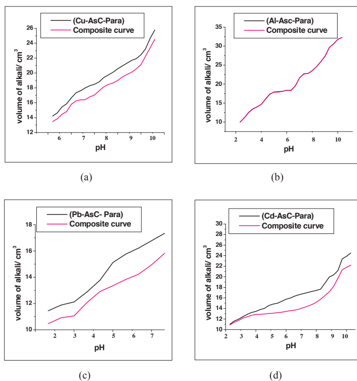
Figure 4: Composite curves and ternary system titration curves of four metal ions :
