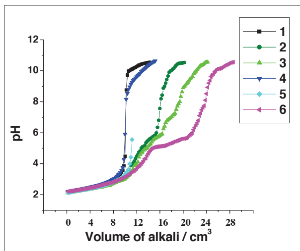
Figure 1: Potentiometric titration curves of binary (1:1) and ternary (1:1:1) complexes of \text{Cu}^{2+} with ascorbic acid and paracetamol; 1) \text{HNO}_3 ; 2) \text{HNO}_3 + ascorbic acid; 3) \text{HNO}_3 + ascorbic acid + \text{Cu}(\text{NO}_3)_2 ; 4) \text{HNO}_3 + paracetamol; 5) \text{HNO}_3 + paracetamol + \text{Cu}(\text{NO}_3)_2 ; 6) \text{HNO}_3 + ascorbic acid + paracetamol + \text{Cu}(\text{NO}_3)_2
