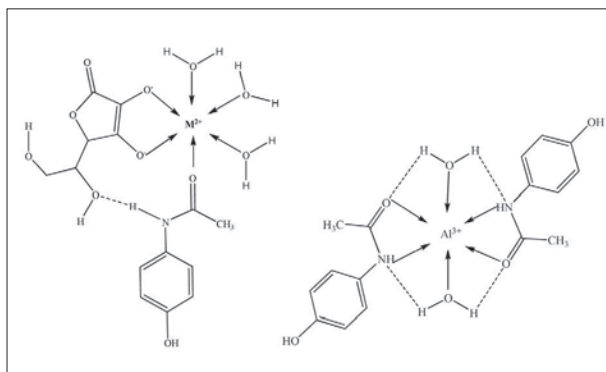
Figure 5: Structure of \text{M(Asc)(Para)} mixed ligand complex ( \text{M} = \text{Pb}^{2+} , \text{Cd}^{2+} , \text{Cu}^{2+} ) and \text{Al(Para)}_2 binary complex
