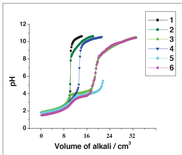
Figure 2: Potentiometric titration curves of binary (1:1) and ternary (1:1:1) complexes of \text{Al}^{3+} with ascorbic acid and paracetamol; 1) \text{HNO}_3 ; 2) \text{HNO}_3 + paracetamol; 3) \text{HNO}_3 + paracetamol + \text{Al}(\text{NO}_3)_3 ; 4) \text{HNO}_3 + ascorbic acid; 5) \text{HNO}_3 + ascorbic acid + \text{Al}(\text{NO}_3)_3 ; 6) \text{HNO}_3 + paracetamol + ascorbic acid + \text{Al}(\text{NO}_3)_3
