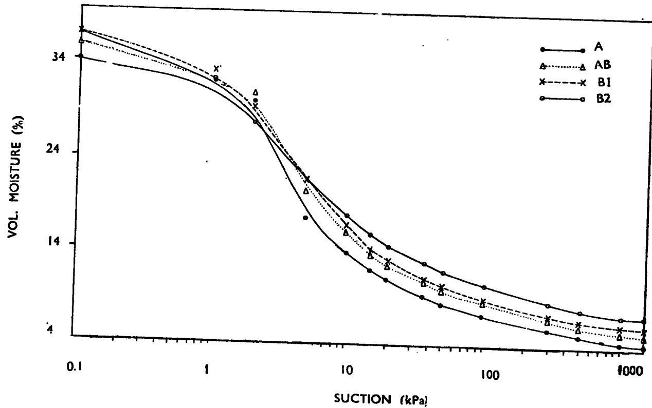
Fig. 1. Soil water retention relationship for major horizons of Non-calcic brown soils.
