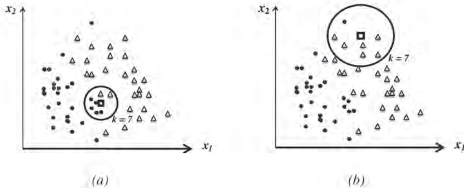
Figure 1: Training feature vector points of a two class problem are represented as \Delta and \bullet . Test point is represented as \blacksquare . (a) In kNN classification, when the concentration of points surrounding the test point is large, a sphere with small radius could enclose seven nearest neighbours. (b) When the concentration of the feature vectors is low, a sphere with larger radius is needed to enclose the seven nearest neighbour points.
