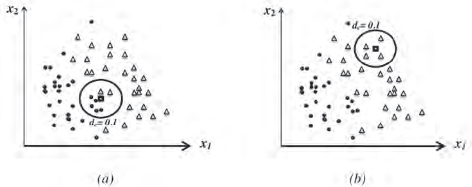
Figure 2: Training feature vector points are as in Figure 1. (a) In FDN classification, when the concentration of points surrounding the test point is large, the sphere with radius d_c encloses large number of neighbours. (b) When the concentration of the feature vectors is low, the sphere encloses fewer numbers of neighbour points.
