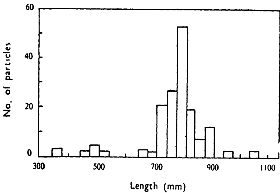
Fig. 2. Histogram of length of virus particles in a leaf squash homogenate (Class interval 133.3 nm)
