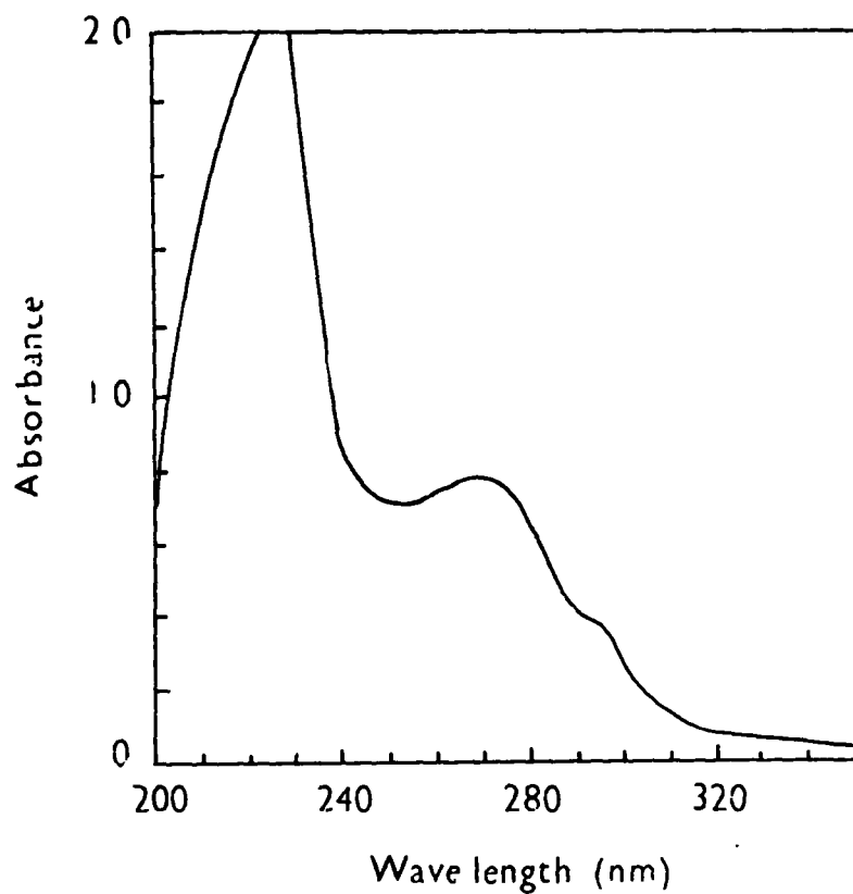
Fig. 1. UV absorption spectrum of purified preparations of passion fruit ringspot virus
