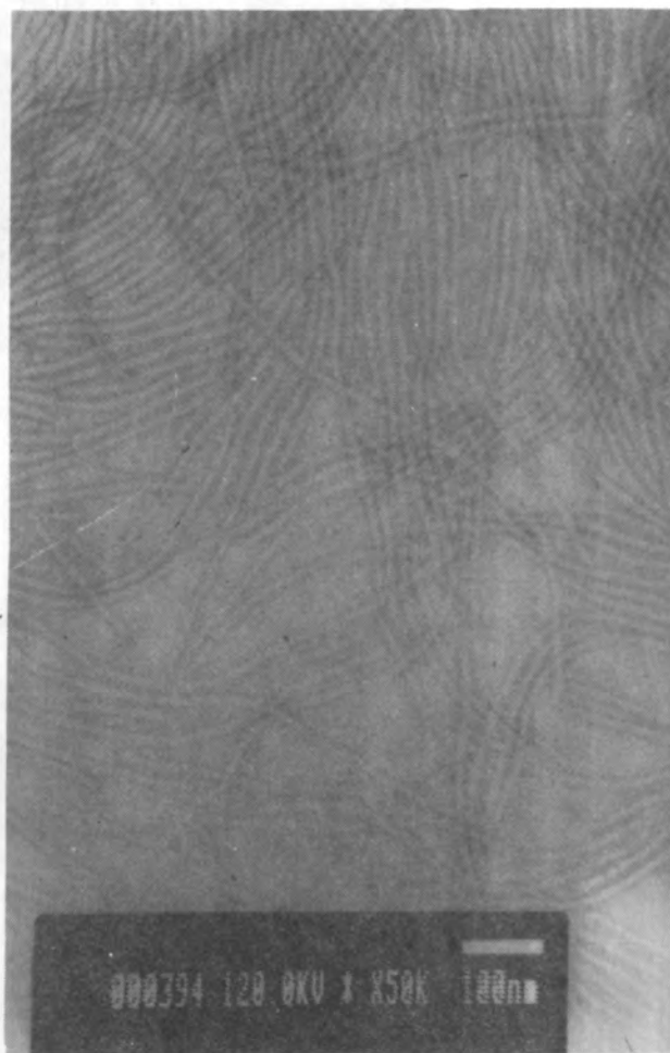
Plate 2. Electron micrograph of purified virus from Passiflora foetida after caesium sulphate density gradient centrifugation, stained in 20 g/l PTA, pH 6.5. Bar represents 100 nm
