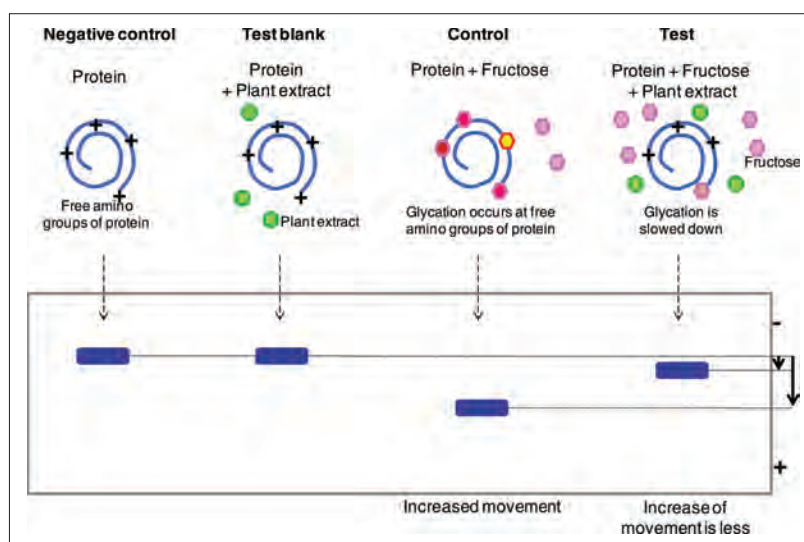
Figure 1: Principle behind the use of PAGE method to detect the protective effects of medicinal plants against protein glycation
