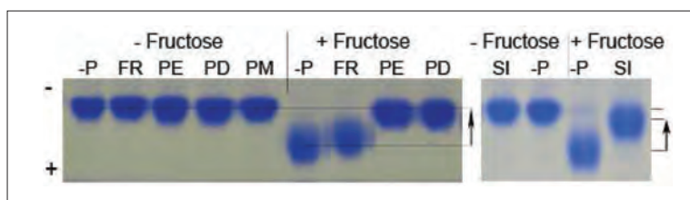
Figure 4: Effect of the presence of plant extracts and standard inhibitor on protein movement
