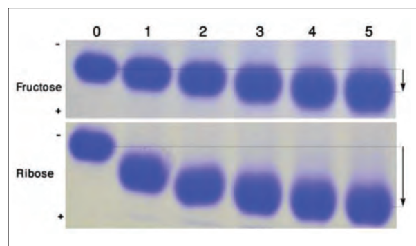
Figure 3: Effect of different sugars (fructose and ribose) and length of incubation (0 – 5 days) on protein movement
