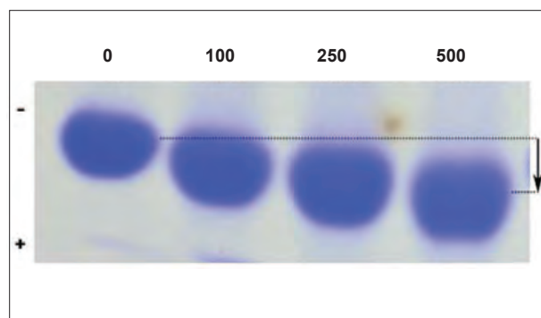
Figure 2: Effect of sugar concentration (0 – 500 mM) on protein movement
