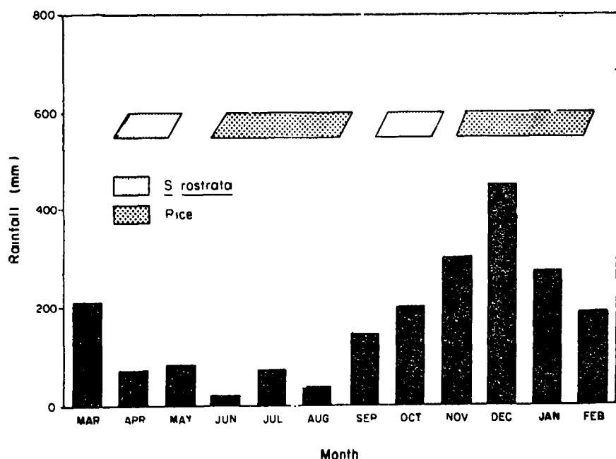
Fig. 3. Depiction of the probable times of growing a 45-day old S. rostrata crop before planting rice (3-3 1/2 month variety) in yala and maha seasons at Girandurukotte
