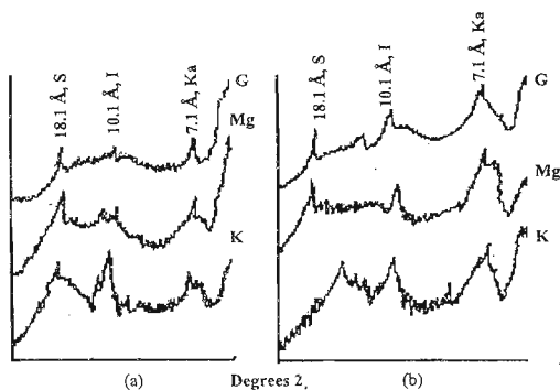
Figure 4: X-ray diffractograms of the clay fraction of Mahailluppallama soil {(a). 0 - 15 cm depth and (b). 15 - 30 cm depth}. Ka = Kaolinite, S = Smectite, I = Illite, K = K-saturated, Mg = Mg-saturated, G = glycerol-solvated.
