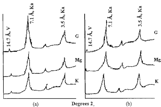
Figure 6: X-ray diffractograms of the clay fraction of Kiribathkumbura soil {(a). 0 - 15 cm depth and (b). 15 - 30 cm depth}. Ka = Kaolin, V = Vermiculite, K = K-saturated, Mg = Mg-saturated, G = glycerol-solvated.
