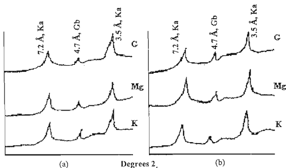
Figure 7: X-ray diffractograms of the clay fraction of Peradeniya soil {(a). 0 - 15 cm depth and (b). 15 - 30 cm depth}. Ka = Kaolin, Gb = Gibbsite, K = K-saturated, Mg = Mg-saturated, G = glycerol-solvated.
