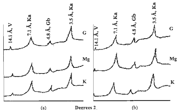
Figure 5: X-ray diffractograms of the clay fraction of Sita Eliya soil {(a). 0 - 15 cm depth and (b). 15 - 30 cm depth}. Ka = Kaolinite, V = Vermiculite, Gb = Gibbsite, K = K-saturated, Mg = Mg saturated, G = glycerol-solvated.
