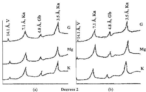
Figure 3: X-ray diffractograms of the clay fraction of Meepilimana soils {(a). 0 - 15 cm depth and (b). 15 - 30 cm depth}. Ka = Kaolin, V = Vermiculite, Gb = Gibbsite, K = K-saturated, Mg = Mg-saturated, G = glycerol-solvated.
