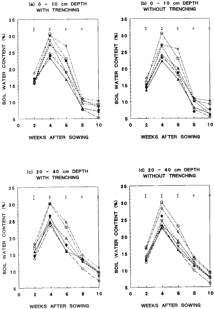
Figure 2: Variation of soil water content (% dry basis) at 0 - 10cm (top soil) and 20 - 40cm (sub-soil) depths under different hedgerow species with and without trenching. \blacktriangle -Calliandra; \triangle -Desmodium; \circ - Flemingia; \bullet - Gliricidia; \diamond - Tithonia; \nabla - Cassia; \square - Control. Vertical bars indicate standard errors at degrees of freedom of 6.
