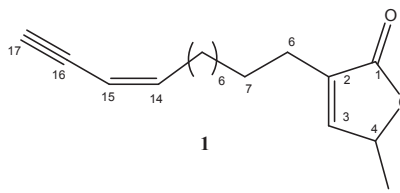
Figure 1: The structure of compound 1
