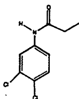
Figure 1: The structure of propanil
