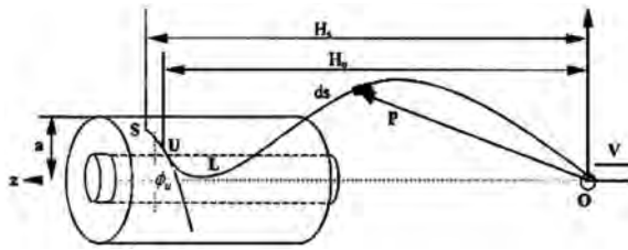
Figure 1: Illustration of over-end unwinding
