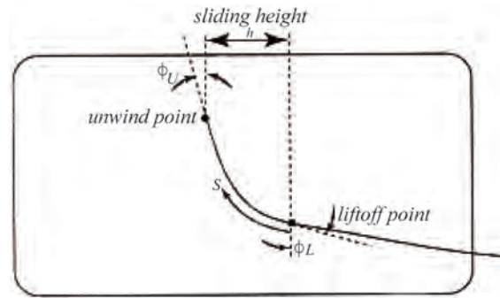
Figure 2: Illustration of drag Region
