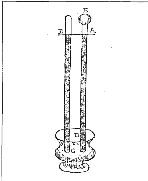
TORRICELLI'S BAROMETER.
