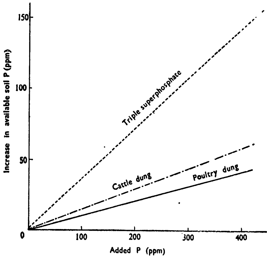
Fig 3. Relationship between increase in available soil P and quantity of P added as animal dung and TSP at 4-week incubation period
