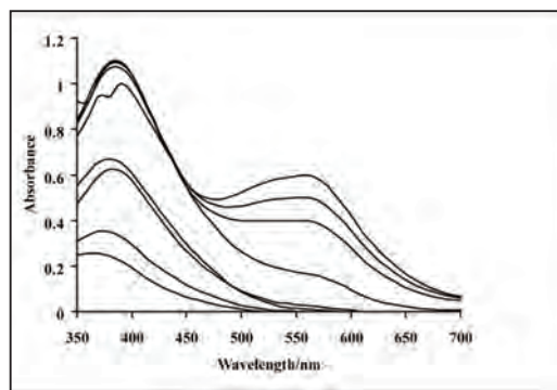
Figure 4.1: Absorption spectra of HT (1.0 mM) as a function of visible light irradiation over 15 hours.
