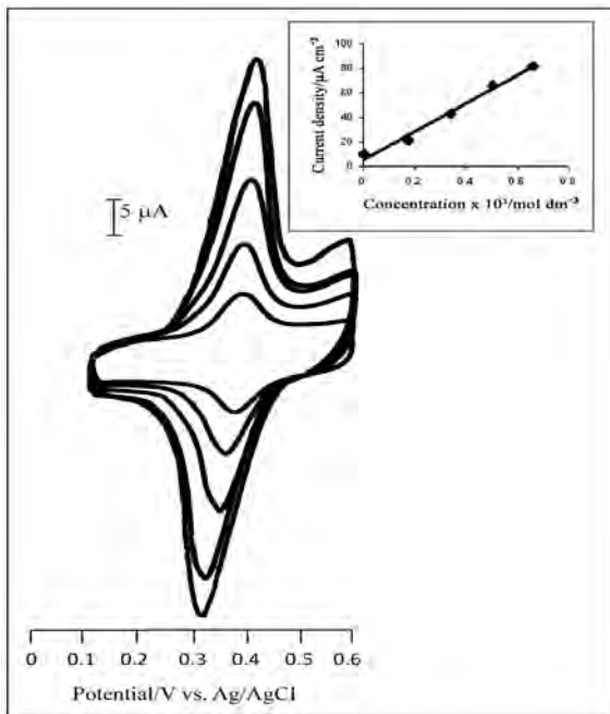
Figure 3: Cyclic voltammograms of HT, when its concentration is varied from 0.005 mM to 0.750 mM in the acetate buffer (pH 4.0) on a glassy carbon electrode at a scan rate of 50 \text{ mV s}^{-1} . The inset shows the plot of current density vs. concentration of HT.
