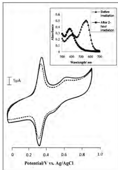
Figure 4.2: Cyclic voltammograms of HT in acetate buffer (pH 4.0) before the irradiation (solid line) and after two hours of irradiation (dashed line), at a scan rate of 50 \text{ mV s}^{-1} . The inset shows the corresponding absorption spectra as a function of time.
