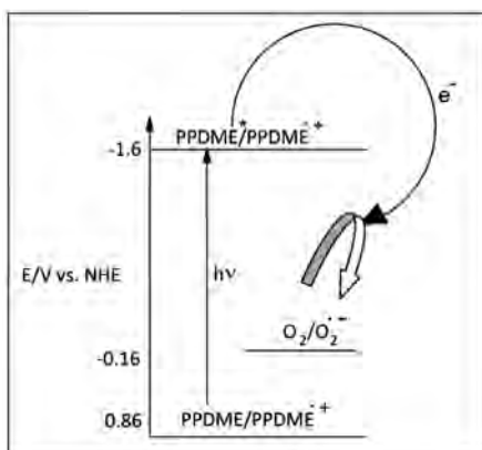
Figure 7: Energy-level diagram showing the formation of superoxide anion through the quenching of excited PPDME by ground state oxygen.
