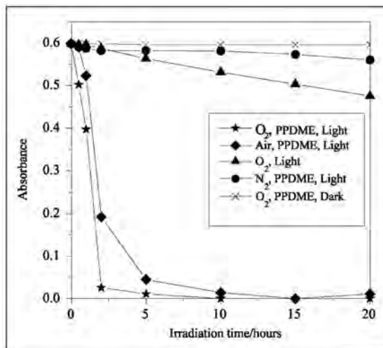
Figure 5: Change in absorbance, measured at 560 nm, for the disappearance of magenta colour of HT, upon irradiation under different conditions.
