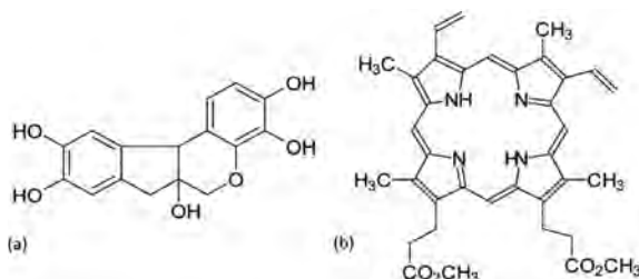
Figure 1: The chemical structure of hematoxylin (a) and protoporphyrin dimethylester (b).
