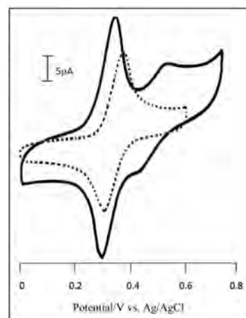
Figure 2: Cyclic voltammograms obtained on a glassy carbon electrode in 0.1 \text{ M} acetate buffer (pH 4.0) containing (a) 0.1 \text{ mM} HT (solid line), (b) 0.2 \text{ mM} catechol (dashed line), at a scan rate of 50 \text{ mV s}^{-1} .
