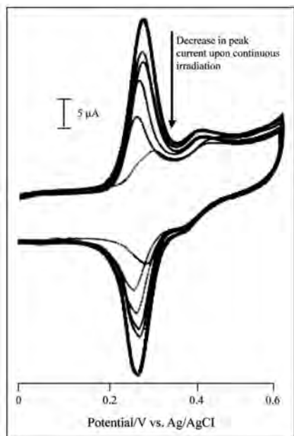
Figure 4.3: Cyclic voltammograms recorded during a 25 hour period of photo-oxidation of HT (0.6 mM) in 0.1 M acetate buffer (pH 4.0), at a scan rate of 50 mV s -1 .
